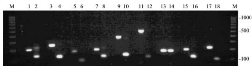
Fig. 1 Agarose gel showing the sizes of gDNA and cDNA amplicons from Heterorhabditis bacteriophora (HP88 strain). A larger gDNA amplification product indicates the presence of introns in the gDNA sequence. M (100 bp DNA ladder). Each pair of numbered lanes shows, respectively, gDNA and cDNA amplification products for a single pair of PCR primers. The PCR primers were as follows: 1–2, F16H9.1a ( rgs-2 ); 3–4, R11A5.4 ( pepck ); 5–6, M106.5 ( cap-2 ); 7–8, T20G5.1 ( chc-1 ) (F1/R1); 9–10, C09B8.1 ( ipp-5 ); 11–12, F08B6.4b ( unc-87 ); 13–14, T20G5.1 ( chc-1 ) (F2/R2), bands of equal size indicating absence of an intron; 15–16, F11C3.3 ( unc-54 ); 17–18, Y54G11 A5a ( cat ). The primer details are presented in Table 1.
